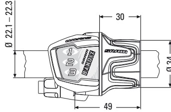
Shifter i-MOTION 3 BANDIX
