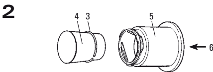
Mounting Tool Part No. 0582 104 000
