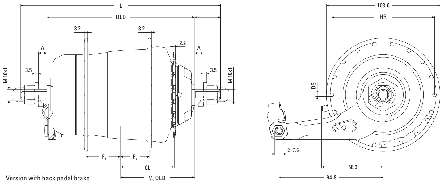
Version with back pedal brake
